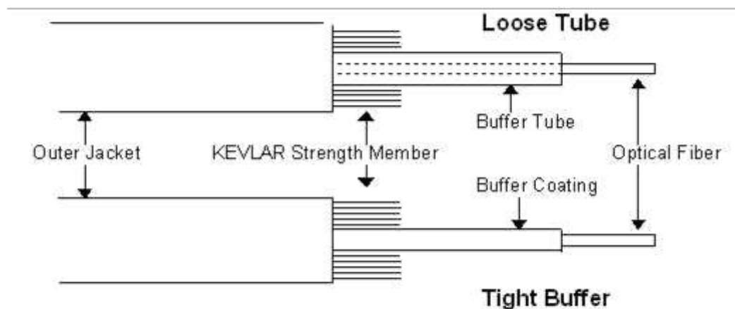
Figure 2, Basic Fiber Optic Cable Construction
