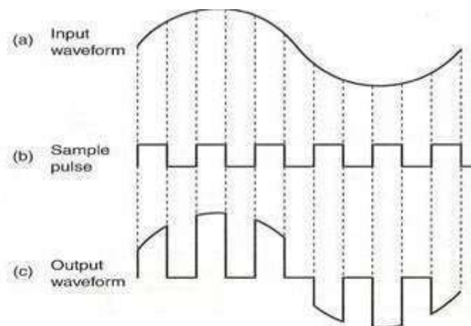
Natural sampling
