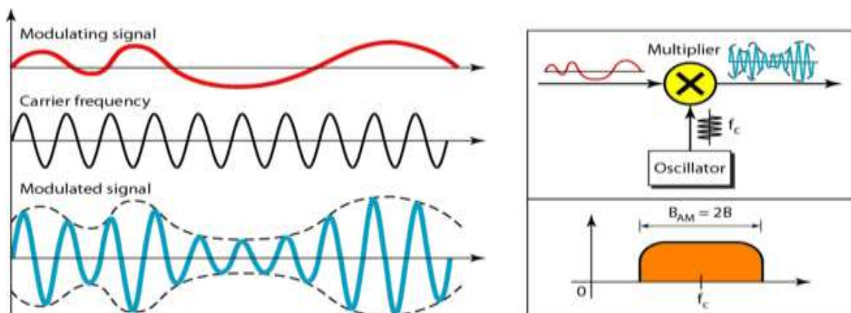
AM generation
