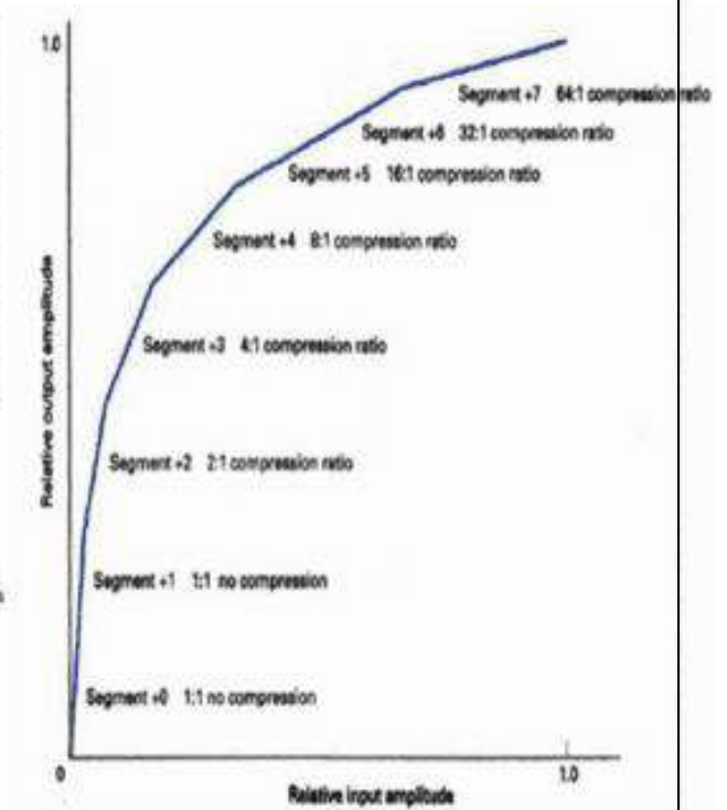
\mu -255compressioncharacteristics
