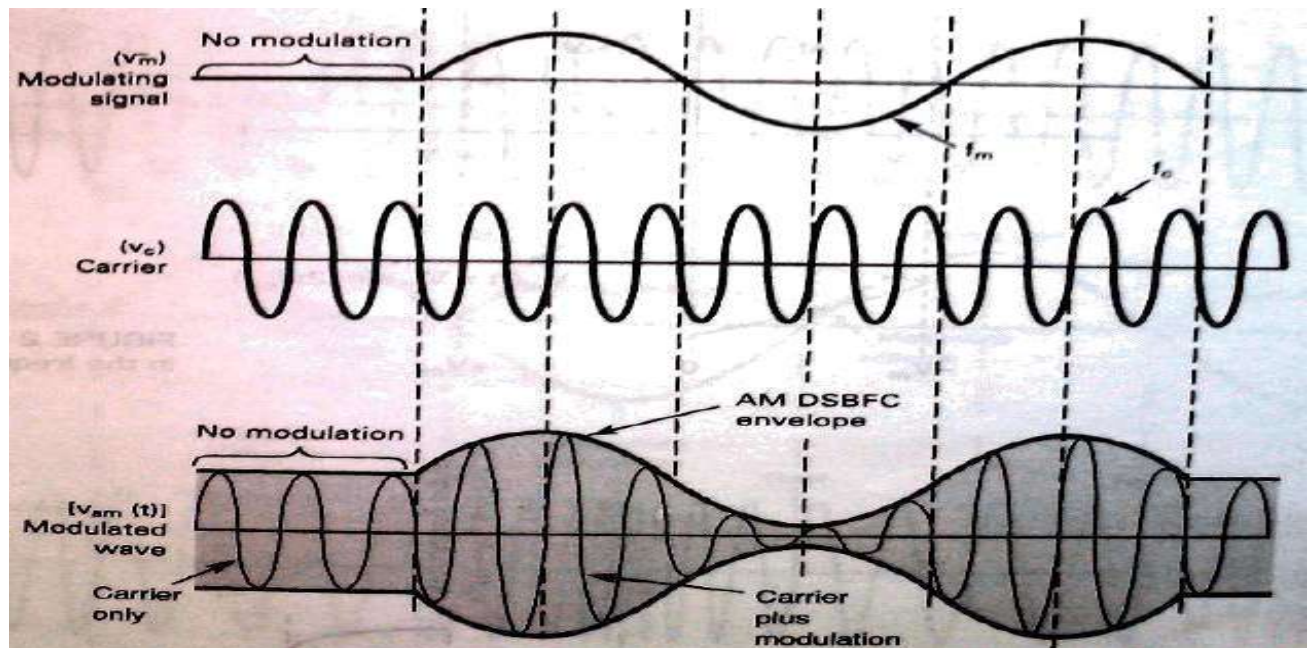
AM generation
