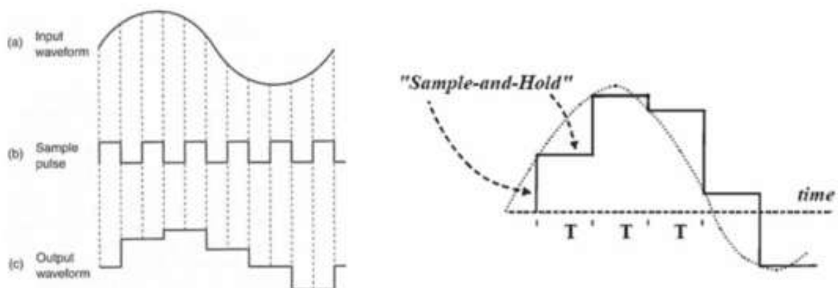
Flat-top sampling
