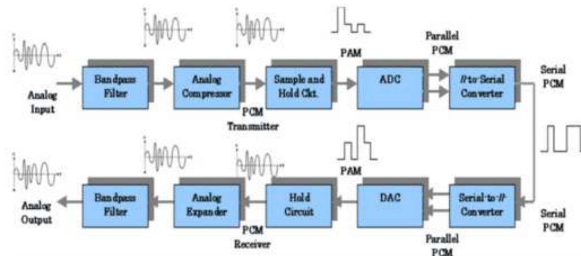
PCM system with analog companding
