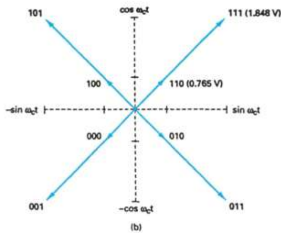
8-QAM modulator: (a) truth table; (b) phasor diagram; (c) constellation diagram
