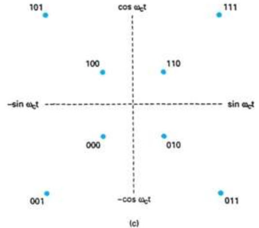
8-QAM modulator: (a) truth table; (b) phasor diagram; (c) constellation diagram
